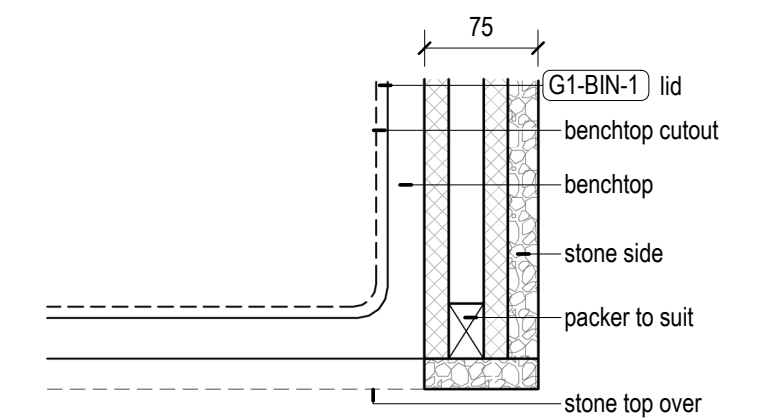
25 Kitchen Island Bin Wall 1 : 5 Plan Detail
