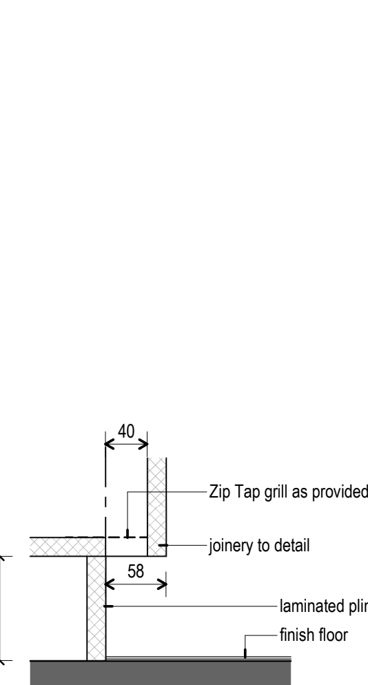
20 Joinery Plinth - Rodent Proof Vent 1 : 5
