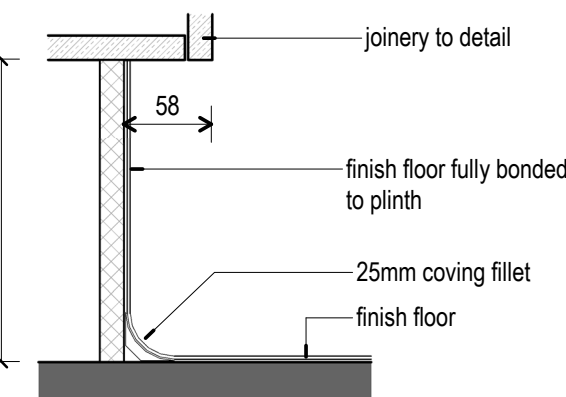
21 Joinery Plinth - Coved Vinyl 1 : 5
