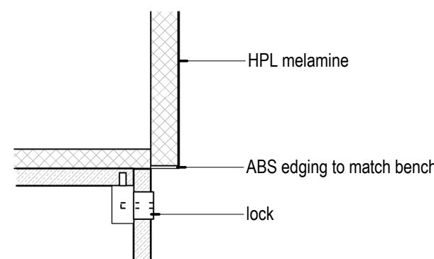
13 Bench Post- Forming 1 : 5
