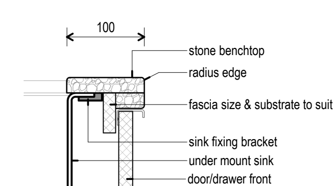
10 Edge Detail - Balance 1 : 5 Stone Benchtop
