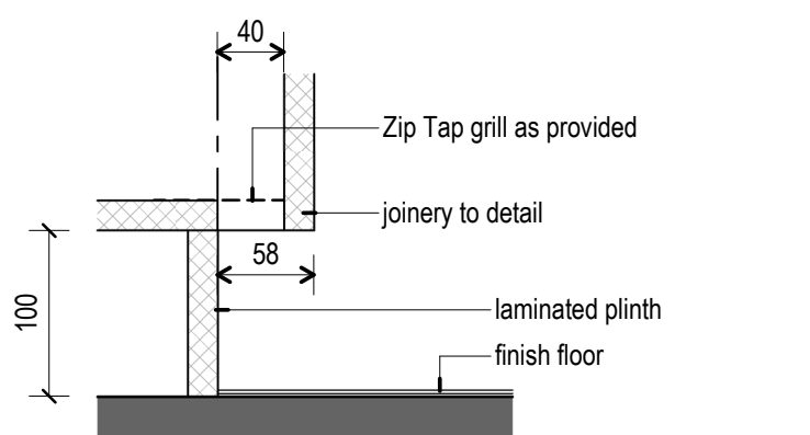
20 Joinery Plinth - Rodent Proof Vent 1 : 5
