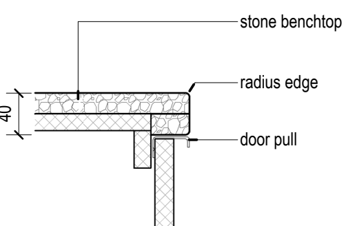
10 Edge Detail - Balance 1 : 5 Stone Benchtop
