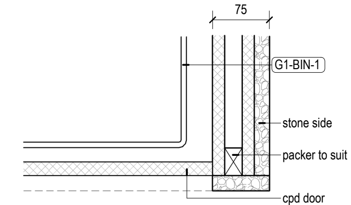
26 Kitchen Island Bin - Door 1 : 5 Plan Detail
