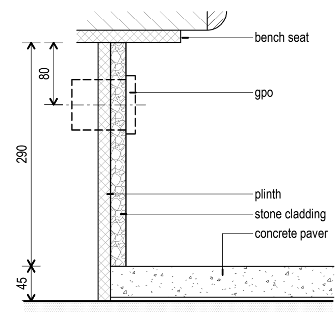
22 JO-SE-1 Plinth 1 : 5
