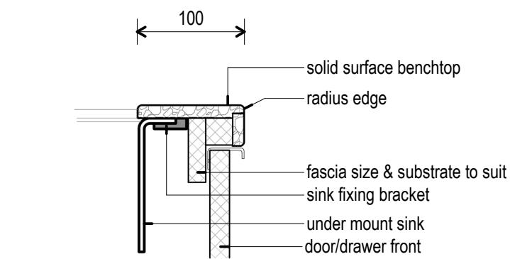
9 Edge Detail - Balance 1 : 5 Solid Surface Benchtop
