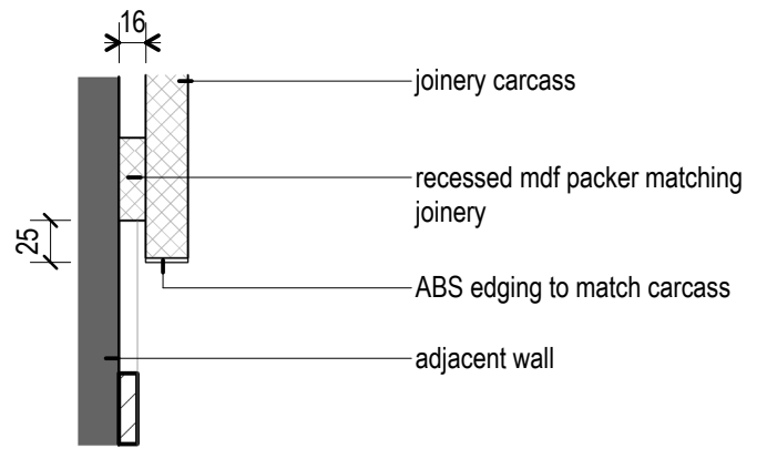
24 Shadowline Detail 1 : 5 Plan Detail
