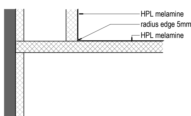
12 Bench Post- Forming 1 : 5
