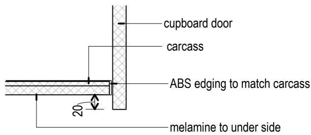
2 Overhead Cpd Shadowline 1 : 5
