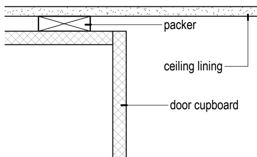
2 Overhead Cpd Shadowline 1 : 5
