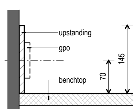
28 Bench Upstanding 1 : 5
