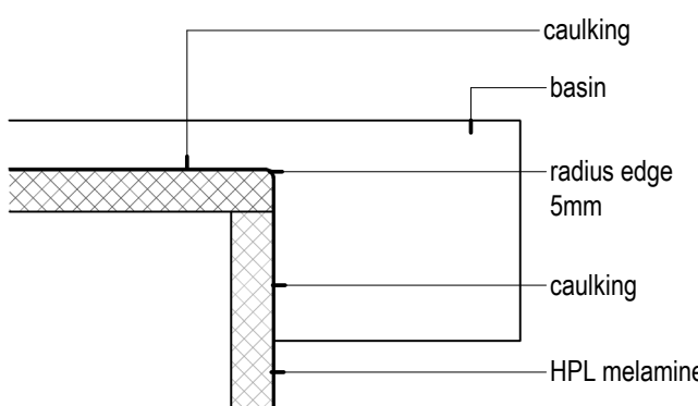
13 Bench Post- Forming 1 : 5
