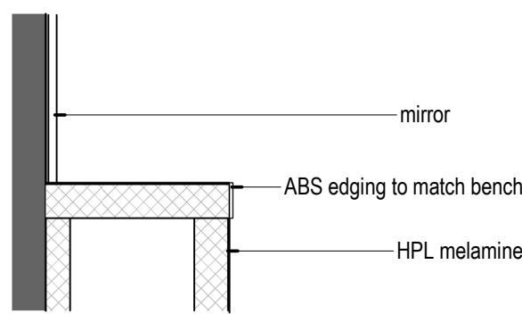
8 Bench Shelf 1 : 5
