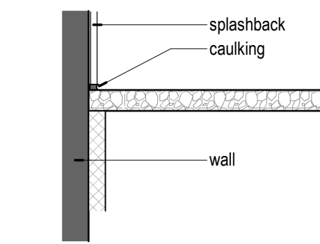
7 Bench to splashback 1 : 5
